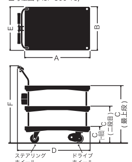
■寸法図 (ASP-300-T3)
