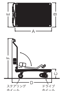
■寸法図 (ASP-300-T3)
